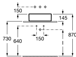
Griferia mural
